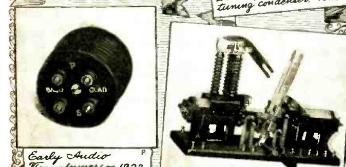
Old-time Army-Navy A.R.C. Changeover Switch - 1916-20
