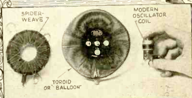
Evolution of tuning coils - 1924-'38 RDW
