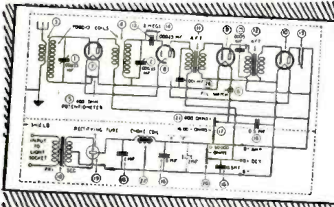
~1926- BATTERYLESS RECEIVER
