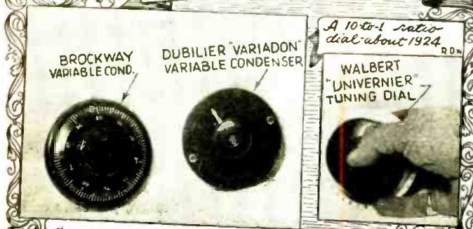
Compression Type Variable Condensers, 1920-24 R.D.W.
