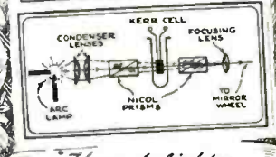
Kerr (light-modulating) cell, and system showing its application, about 1931.
