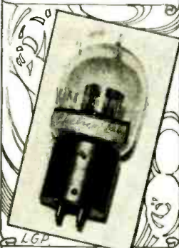
Electron Relay (Moorehead) - 1925-22.
