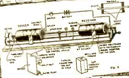
Early image receiver and transmitter - about 1927.
