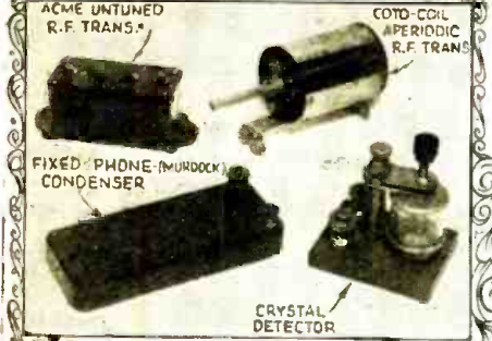
Early Radio Parts from 1912-1923. R.D.W.
