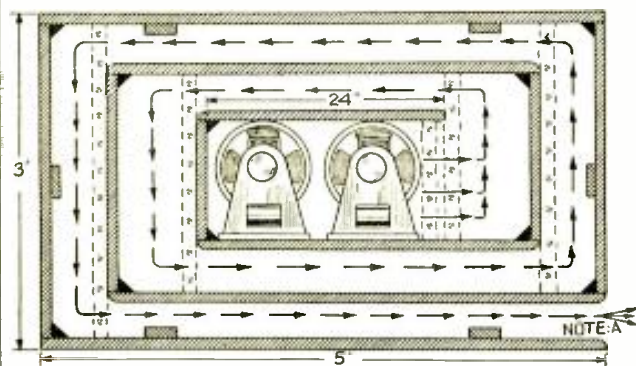
Fig. 17. Constructional data for the infinite-baffle cabinet housing the 2 speakers.
