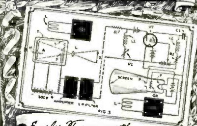
Early Farnsworth cathode-ray television transmitting and receiving system, about 1931.
