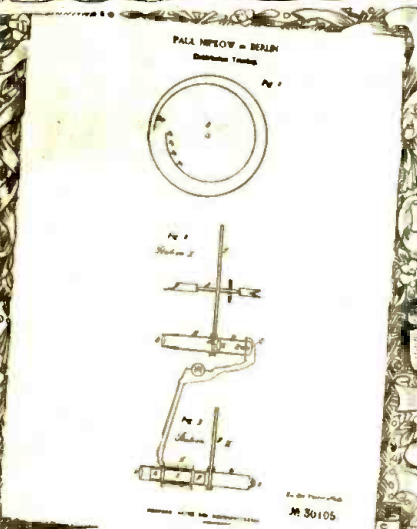
Reproduction of patent drawing of Nipkow's Scanning Disc - 1884.
