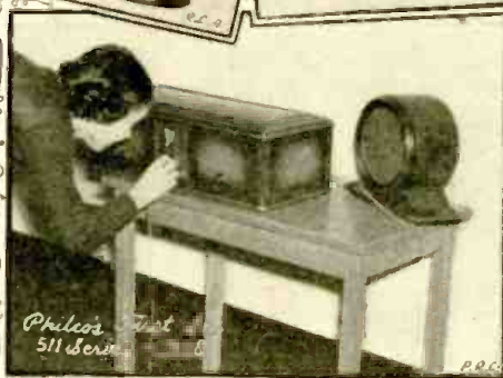
6-Tube TRF, Low-Loss Resistance Coupled Set, with Electrostatic Shielded Oscillation Suppressors - about 1925
